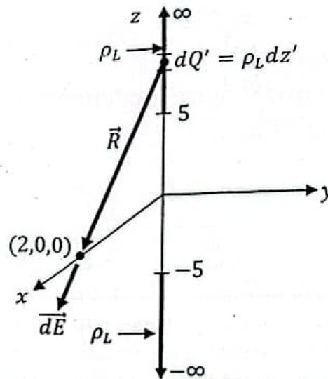
Figure 2. Two semi-infinite line charges on z -axis
